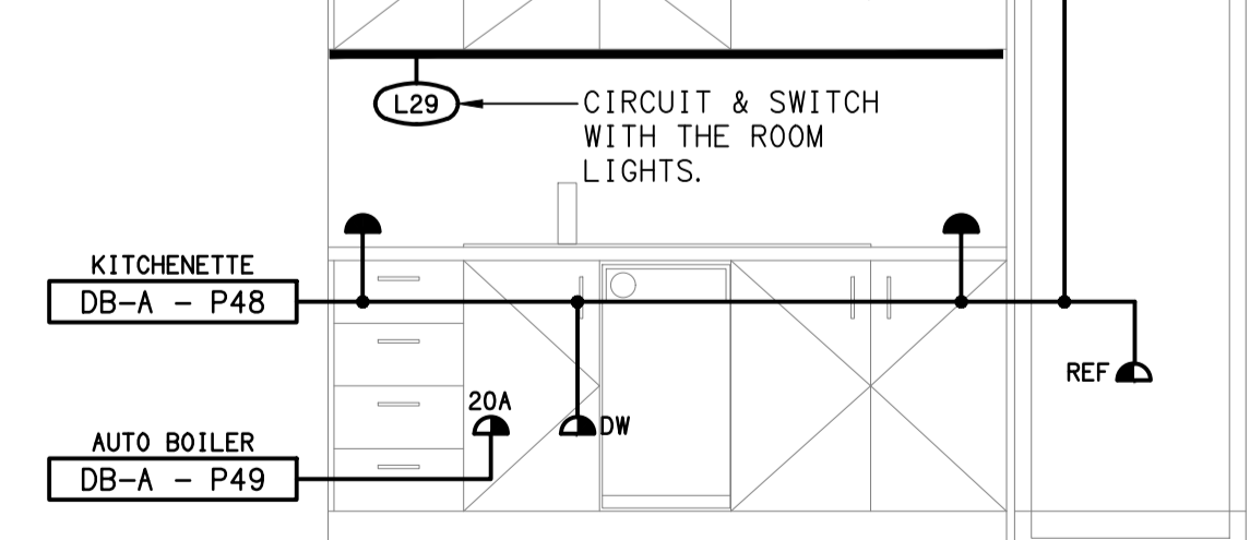
DETAIL A WORK AREA KITCHENETTE ELEVATION SCALE 1:25
